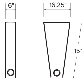
Straight & Wedge Arm Connectors
