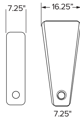
Straight & Wedge Arm Connectors
